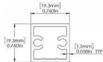
D 5 MIDDLE (PINNED) BALUSTER NOT-TO-SCALE
