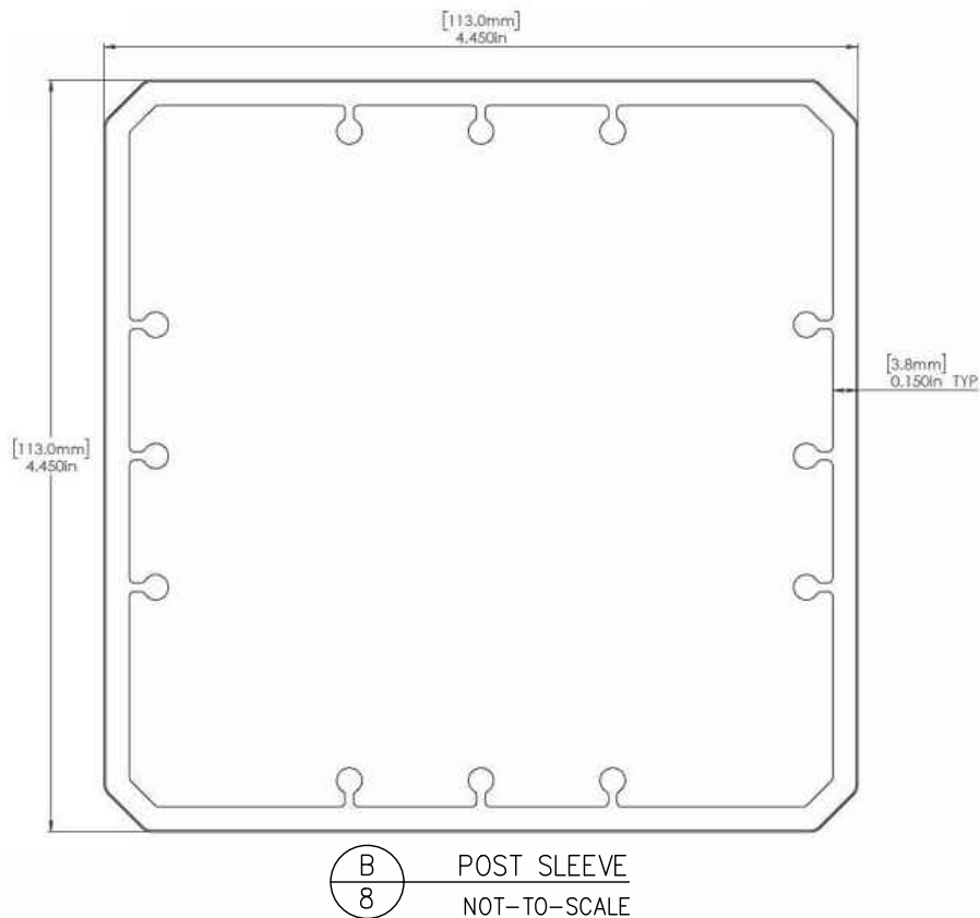
POST MOUNT SPACER NOT-TO-SCALE
